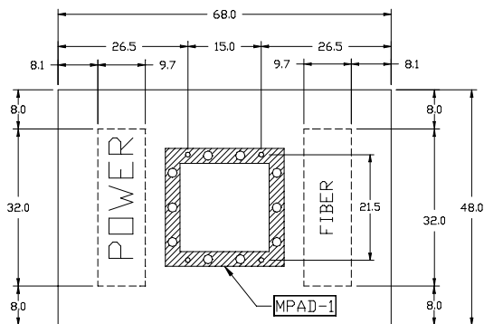
Pad Mounting Template with Frame
