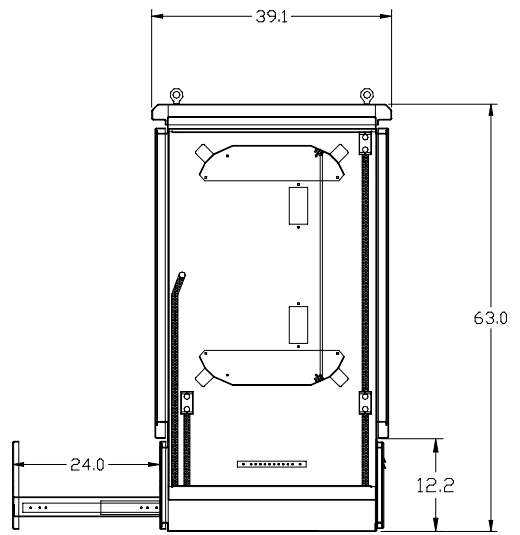
Fiber Storage Compartment
