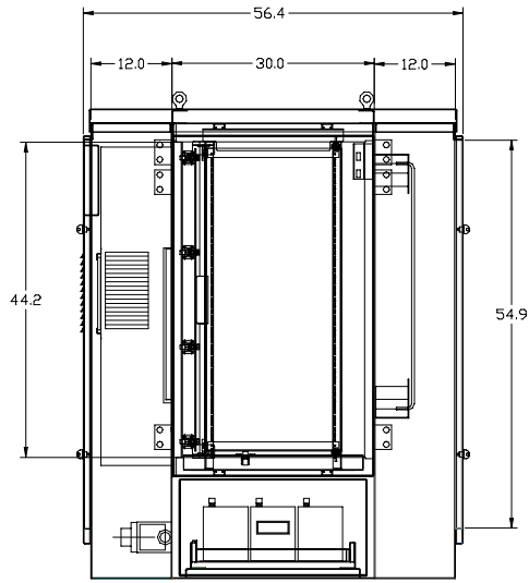
MCCES1 Front View
