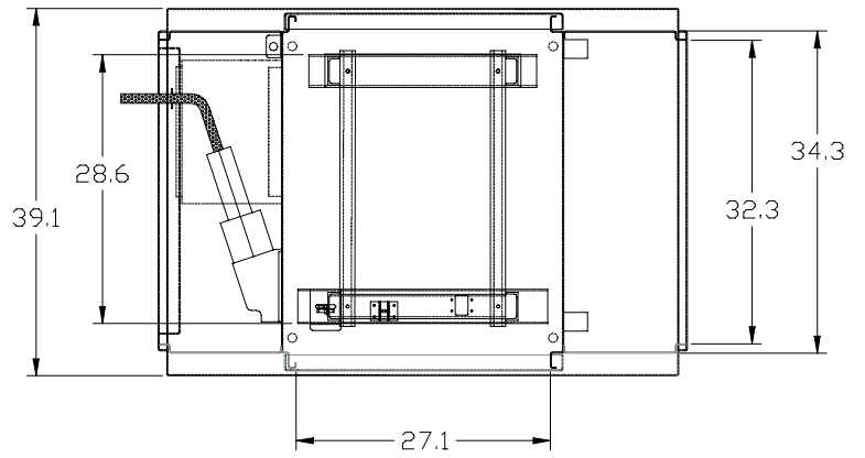
MCCES1 Top View
